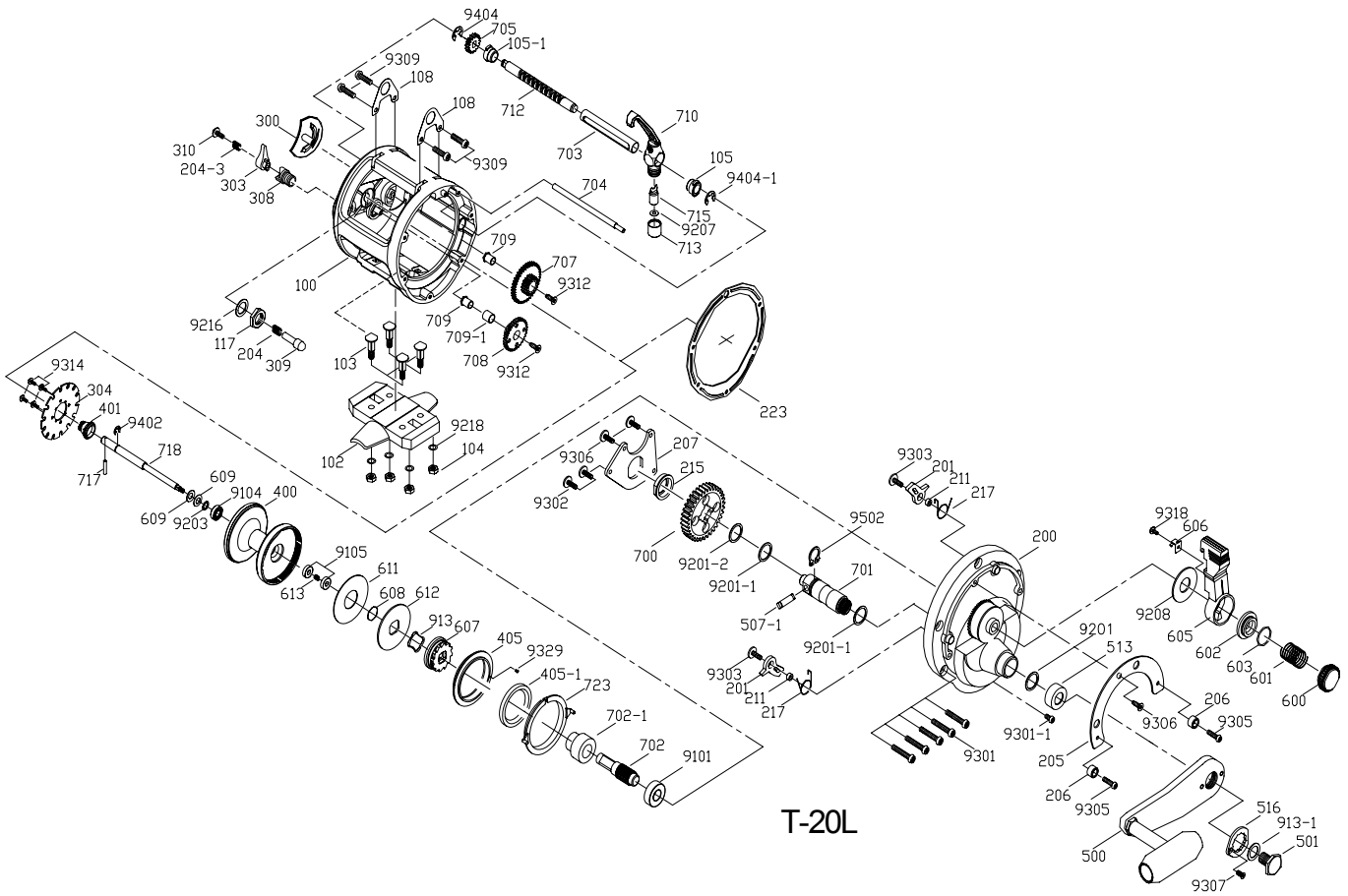
T - 20L (1 of 2) Spare Parts
